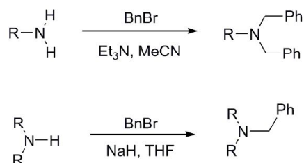
Scheme 1. Protection of amine using benzyl bromide or benzyl chloride
