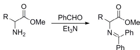
Scheme 6. Protection of amine using benzaldehyde and triethyl amine
