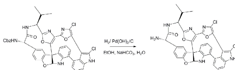
Scheme 15. Deprotection of N-Cbz bond by \text{H}_2/\text{Pd}(\text{OH})_2
