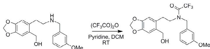
Scheme 12. Protection of amine by trifluoroacetic anhydride
