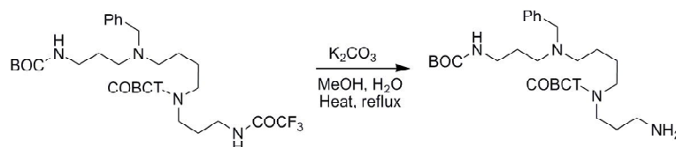
Scheme 13. Deprotection of N-trifluoroacetyl bond using K_2CO_3
