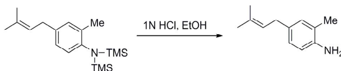
Scheme 9. Deprotection of N-trimethylsilyl bond using HCl in ethanol
