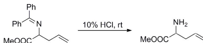
Scheme 7. Deprotection of N-Benzylideneamine bond using 10% HCl
