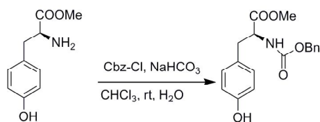
Scheme 14. Protection of amine by benzyloxycarbonyl chloride
