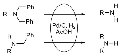
Scheme 2. Hydrogenolysis of benzylamines
