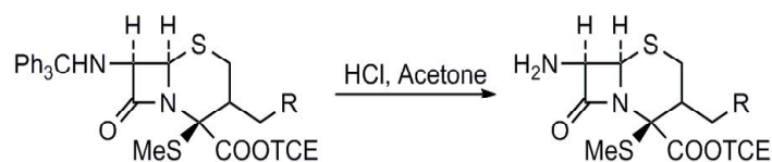
Scheme 5. Cleavage of N-trityl bond using HCl
