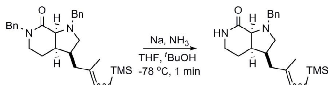
Scheme 3. Cleavage of N-Benzyl bond using Sodium in liquid ammonia
