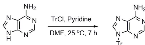
Scheme 4. Protection of amine using Trityl Chloride and base
