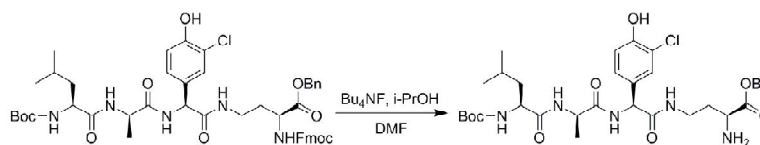
Scheme 19. Deprotection of N-Fmoc by Bu 4 NF
