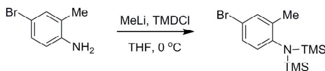
Scheme 8. Protection of amine using Trimethylsilyl chloride
