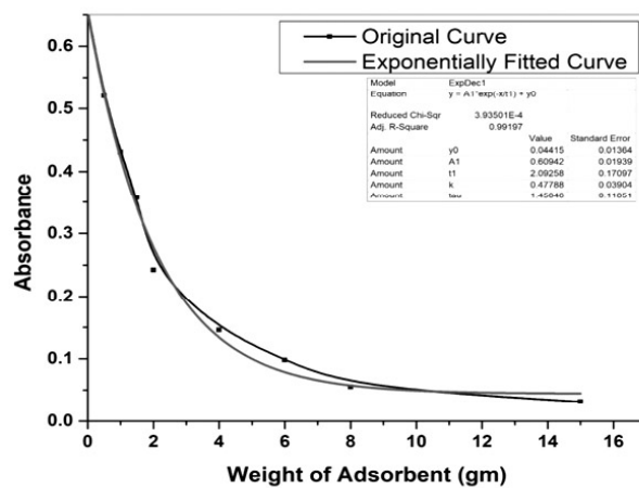
Figure 6. Change of absorption value of \text{KMnO}_4 with increase in the weight of coconut coir adsorbent.
